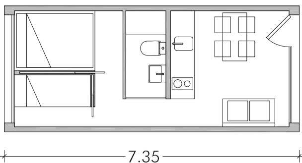
ref. ED01.3173.CX.02C Bungalow/mobile home adossat 2 habitacions
